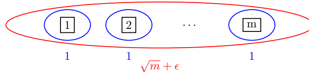
Figure 4: Challenge instance for Greedy-by-Sqrt-Value-Density
